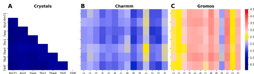
Fig. 10. RMSD analysis (for binding site residues) of RdRp ensembles. (A) All-against-all root-mean-square deviation (RMSD) between conformations included in the RdRp Crystal ensemble (i.e., experimental data). (B) RMSD of all conformations of the RdRp Charmm ensemble (x-axis) against all conformations of the RdRp Crystal ensemble (y-axis). (C) RMSD of all conformations of the RdRp Gromos ensemble (x-axis) against all conformations of the RdRp Crystal ensemble (y-axis). All RMSD values were computed using all the heavy atoms of residues in the catalytic binding site. The range bar on the right, with RMSD values in Angstroms, indicates the color code used in all three plots.
